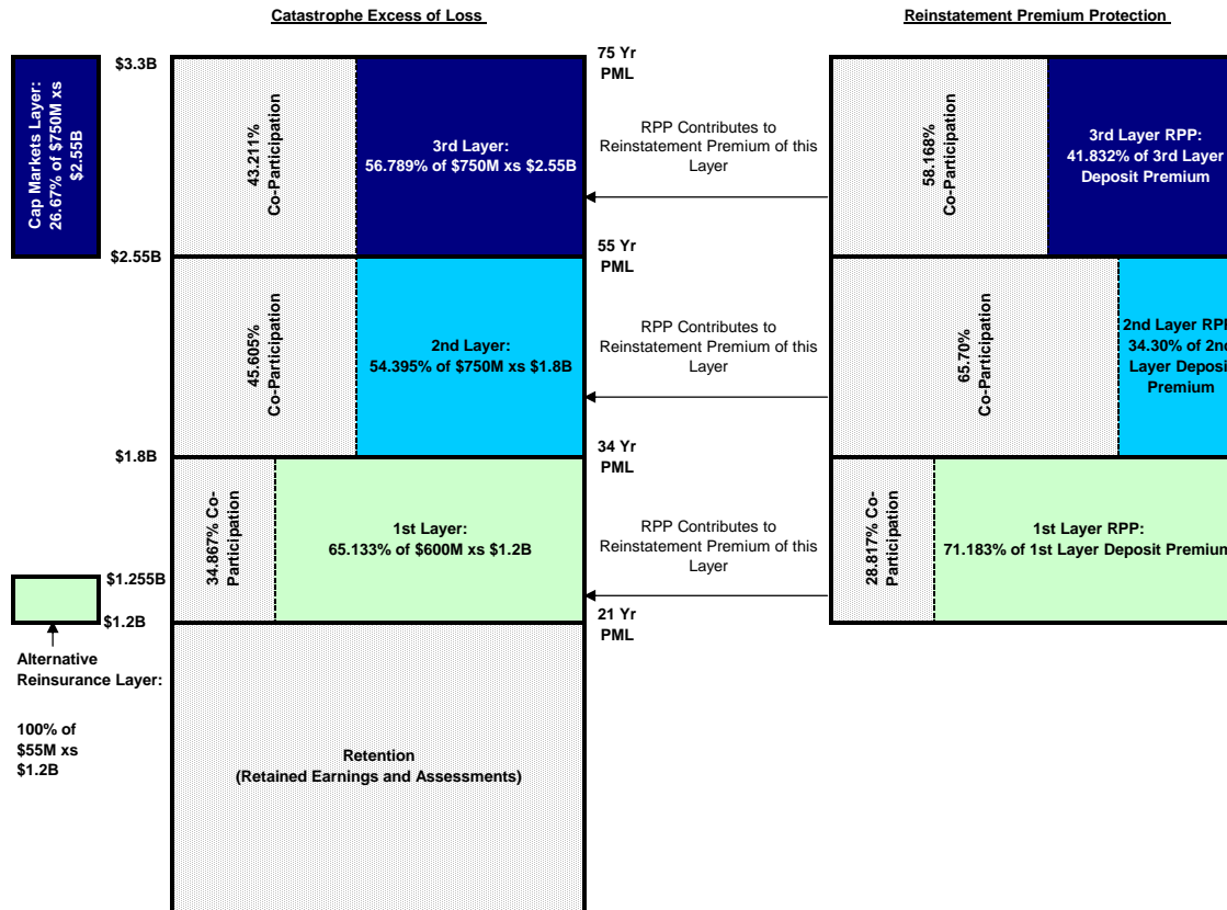
Structure Graph
